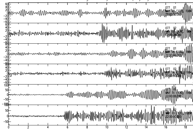
DSS waveforms digitized by DGS. Display by SAC
