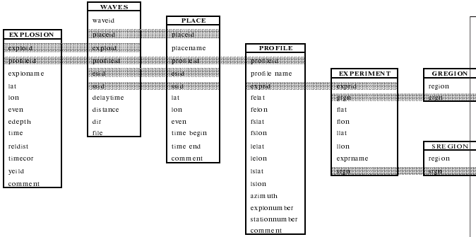
Deep Seismic Sounding Database Structure Highlights
